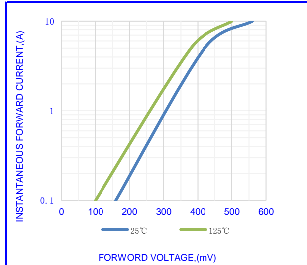
Fig.2-TYPICAL INSTANTANEOUS FORWARD
