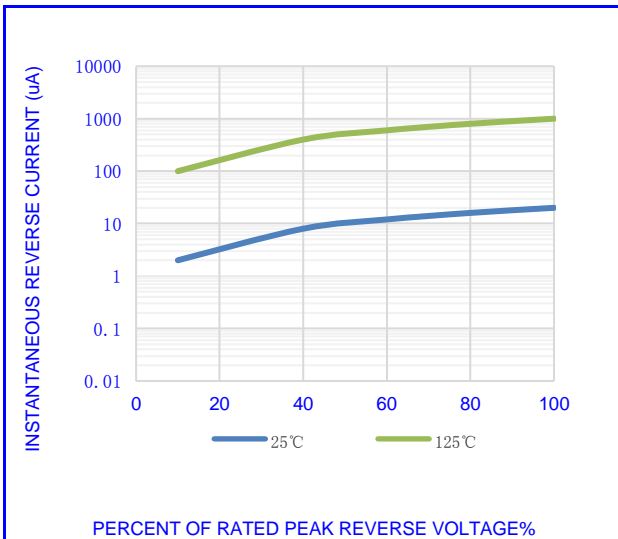
Fig.3-TYPICAL REVERSE CHARACTERISTICS
