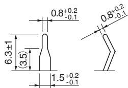
(Terminal dimensions)
