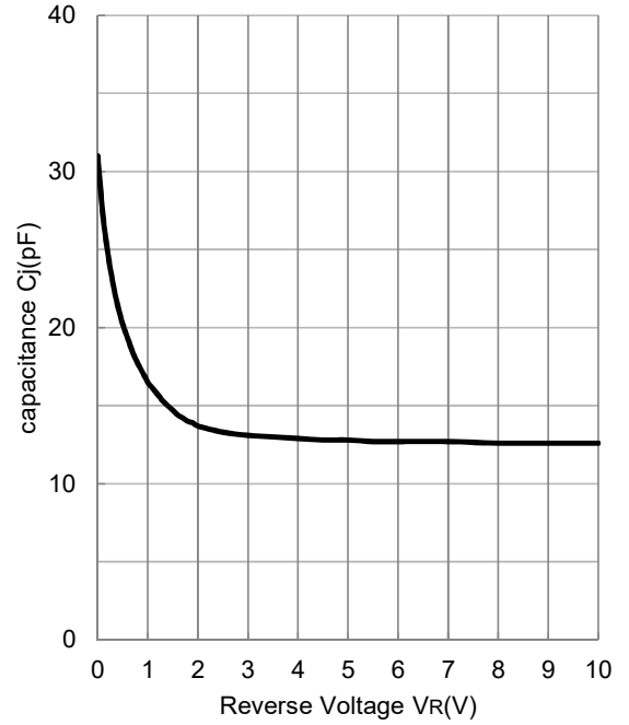
capacitance vs. Reverse Voltage (Ta=25°C)
