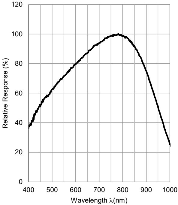
Spectral Response (Ta=25°C) Detector
