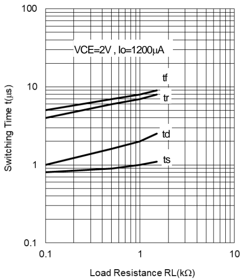
Switching Time vs. Load Resistance (Ta=25°C)
