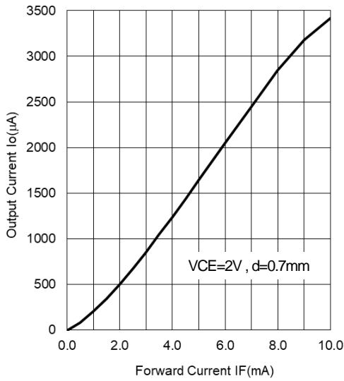
Output Characteristics (Ta=25°C)
