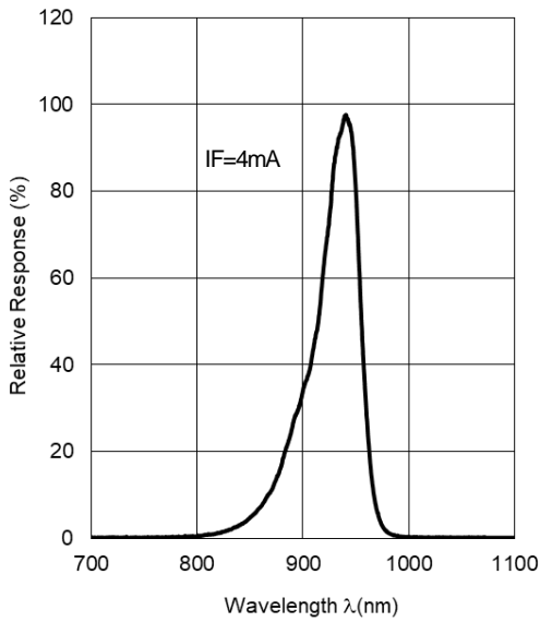
Spectral Response (Ta=25°C) Emitter
