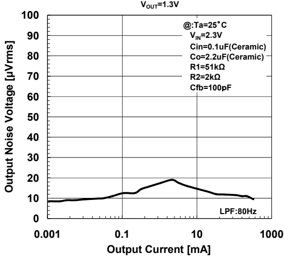
Output Noise Voltage vs. Output Current
