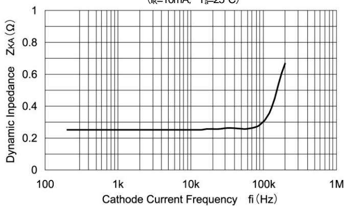
Dynamic Impedance
