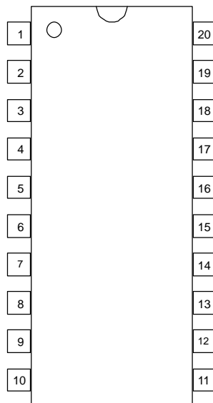
NJM2625AD NJM2625AM
