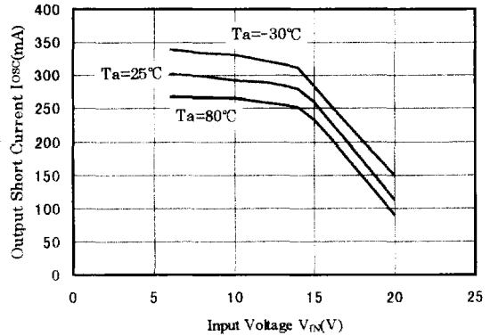
Output Short Current vs. Input Voltage
