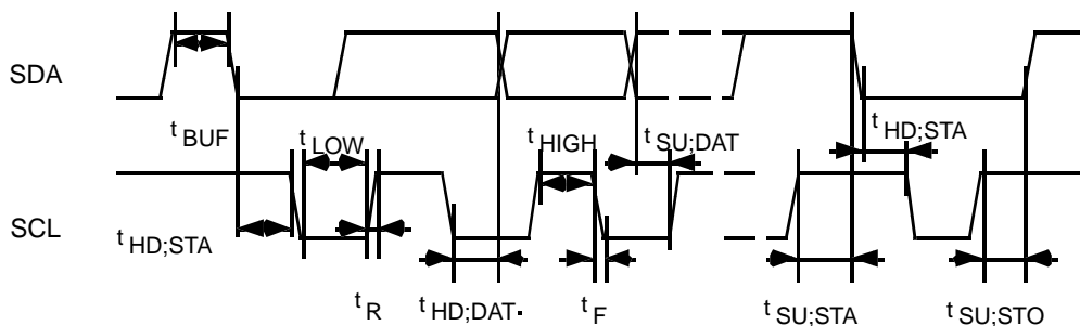
I 2 C bus Timing Chart V IHmin (0.7 Vcc1) and V ILmax (0.3 Vcc1)
