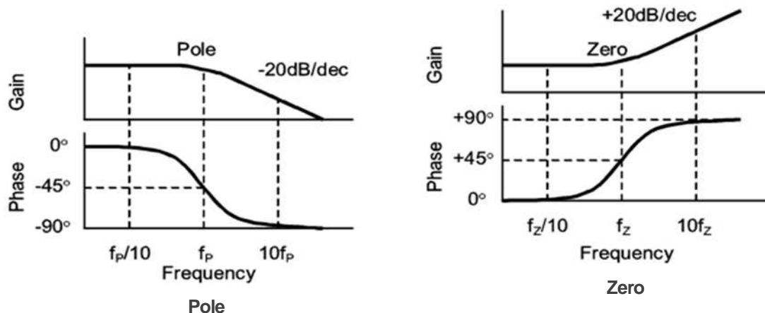
Figure 9. Pole and Zero Characteristics
