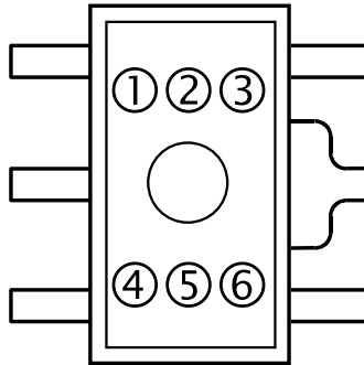
SOT-89-5 Mark Specification
