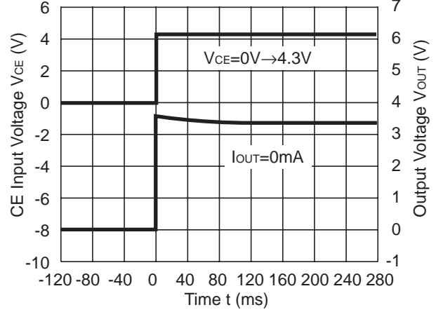
R1161x33xx (ECO=L)
