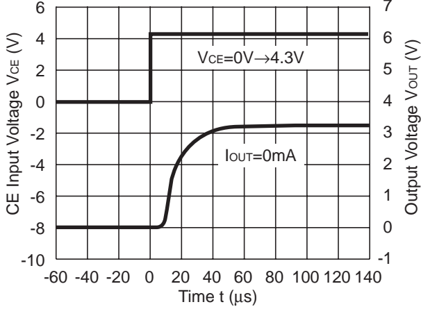
R1161x33xx (ECO=H)
