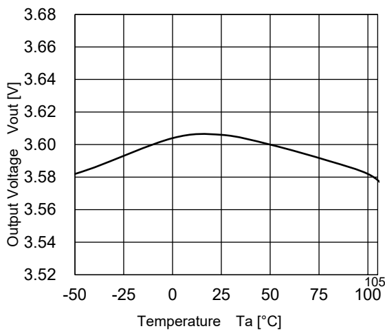
R1180x361x ( V_{IN}=4.6V )
