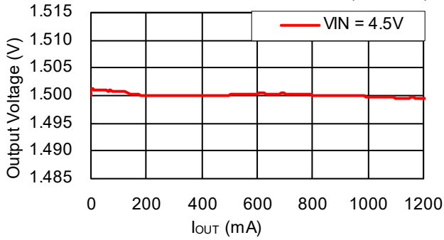
R1245x00xG/R1245x00xH V_{OUT}=1.5V
