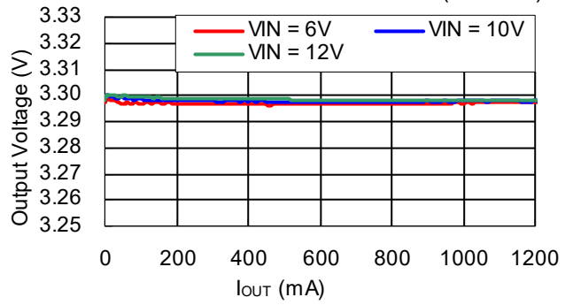
R1245x00xG/R1245x00xH V_{OUT}=3.3V
