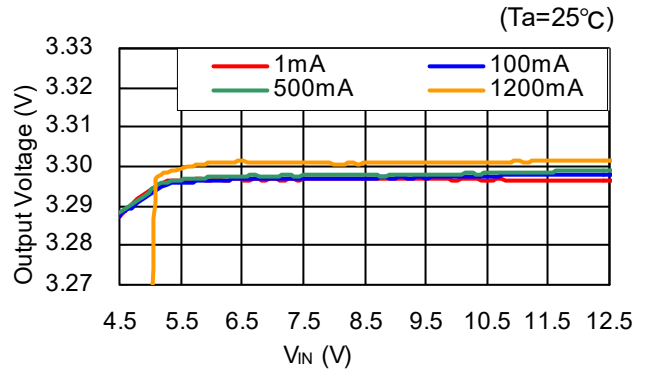
R1245x00xG/R1245x00xH V_{OUT}=3.3V
