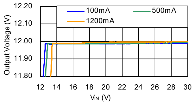
R1245x00xC/R1245x00xD V_{OUT}=12V
