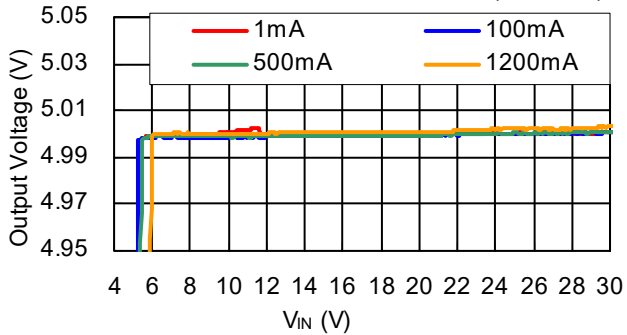
R1245x00xC/R1245x00xD V_{OUT}=5.0V
