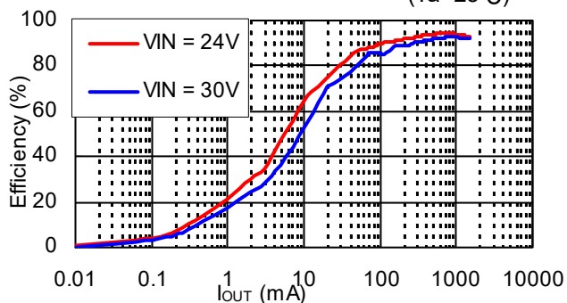
R1245x00xE/R1245x00xF V OUT =15V
