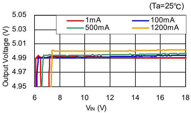
R1245x00xG/R1245x00xH V_{OUT}=5.0V
