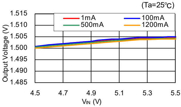
R1245x00xG/R1245x00xH V_{OUT}=1.5V
