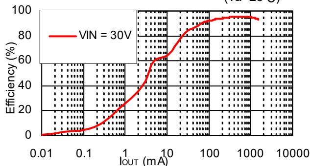
R1245x00xE/R1245x00xF V OUT =24V
