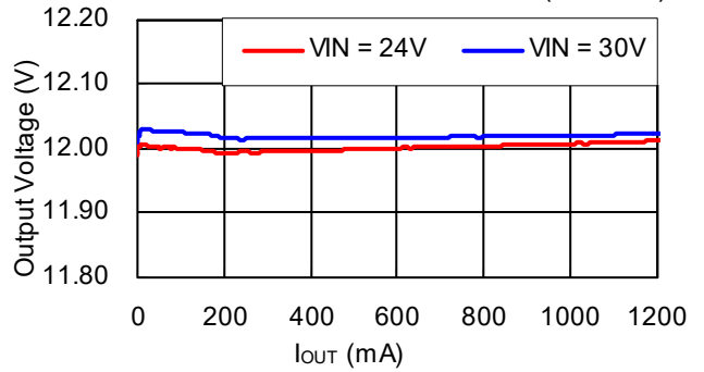
R1245x00xG/R1245x00xH V_{OUT}=12V
