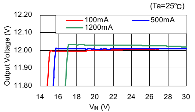
R1245x00xG/R1245x00xH V_{OUT}=12V
