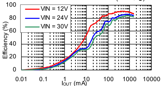
R1245x00xE/R1245x00xF V OUT =5.0V
