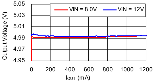
R1245x00xG/R1245x00xH V_{OUT}=5.0V
