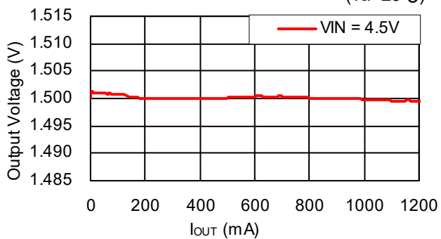
R1245x00xG/R1245x00xH V_{OUT}=1.5V
