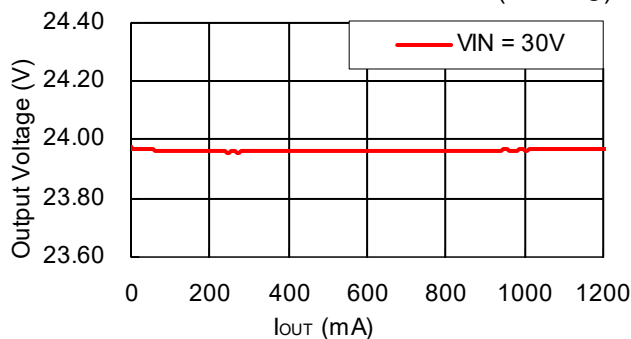
R1245x00xC/R1245x00xD V_{OUT}=24V
