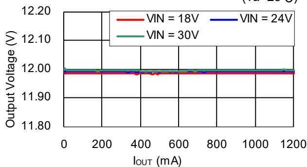
R1245x00xC/R1245x00xD V_{OUT}=12V
