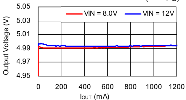
R1245x00xG/R1245x00xH V_{OUT}=5.0V
