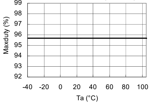
R1245x00xC/R1245x00xD ( V_{IN} = 12V )
