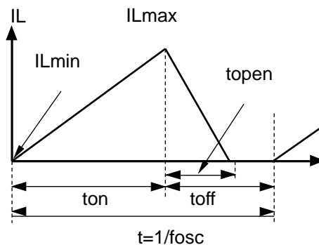
Current flowing through the Inductor
