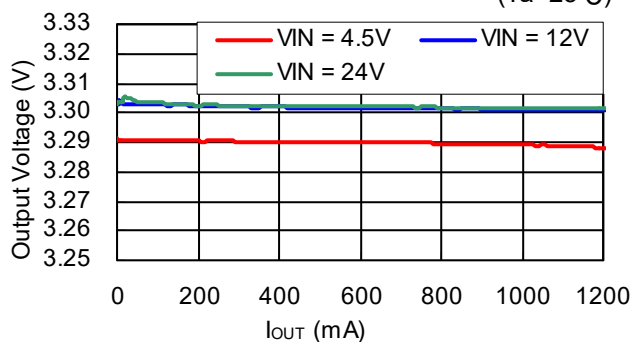
R1245x00xC/R1245x00xD V_{OUT}=3.3V
