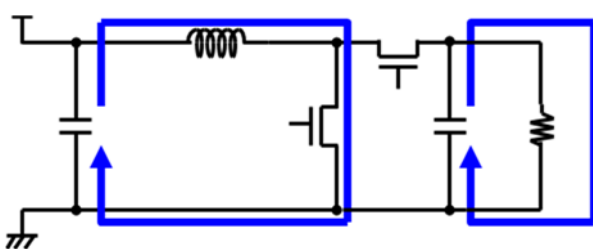
NMOSFET-ON (BOOST)
