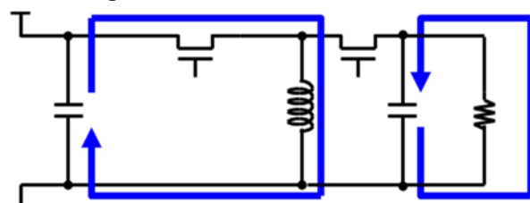
PMOSFET-ON (INVERTING)
