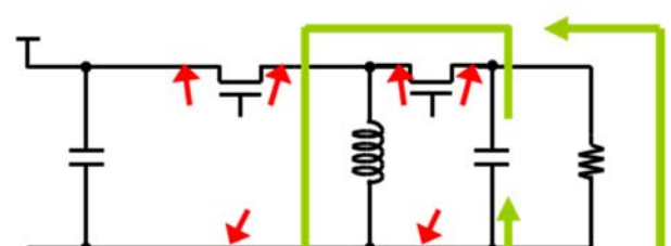
NMOSFET-ON (INVERTING)
