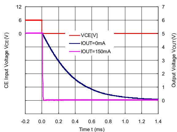
R1517x50xF (C2 = 0.1 μF, CD = 1 nF)
