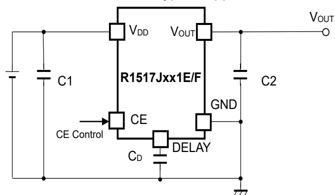
R1517xxxxE/F Typical Application
