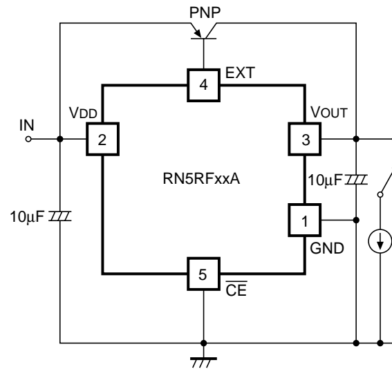
Test Circuit for Load Transient Response
