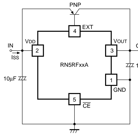
Test Circuit for Supply Current
