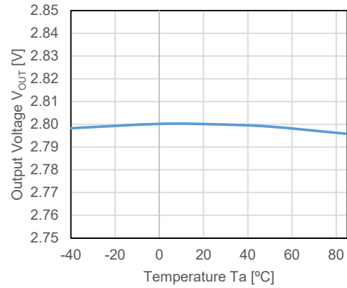
RP122x28xx, V_{IN} = 3.8 V, I_{OUT} = 1 mA
