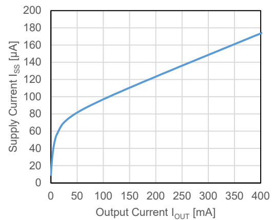
RP122x28xx, V_{IN} = 3.8 \text{ V}
