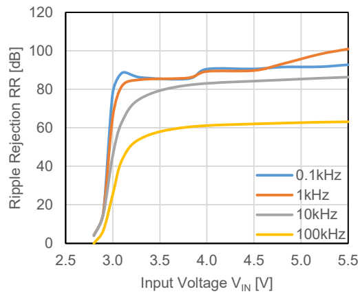
RP122x48xx, I OUT = 100 mA
