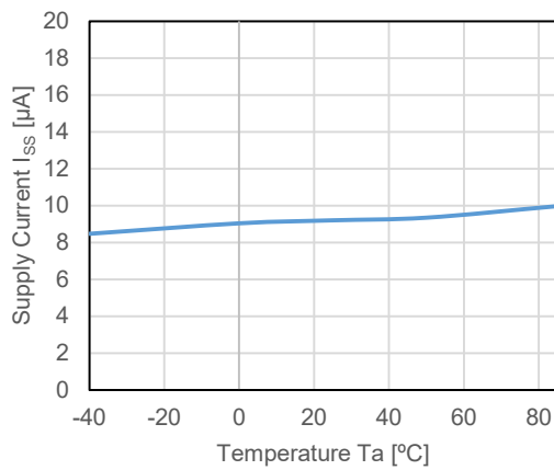
RP122x12xx, V_{IN} = 2.2 V
