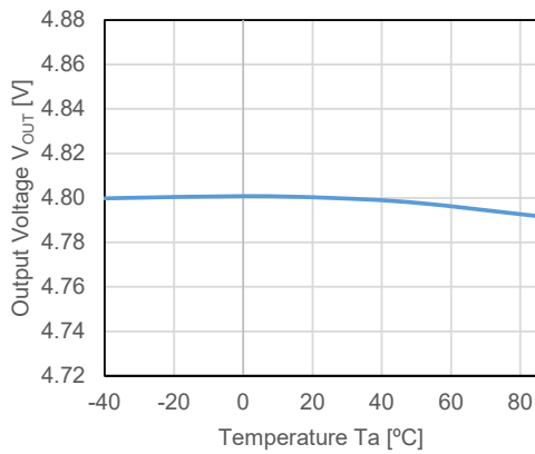
RP122x48xx, V_{IN} = 5.5 V, I_{OUT} = 1 mA
