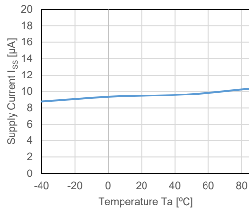
RP122x28xx, V_{IN} = 3.8 V
