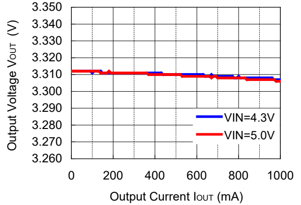
RP505K V_{OUT}=3.3V
