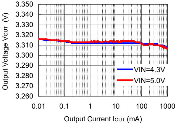
RP505K V_{OUT}=3.3V
