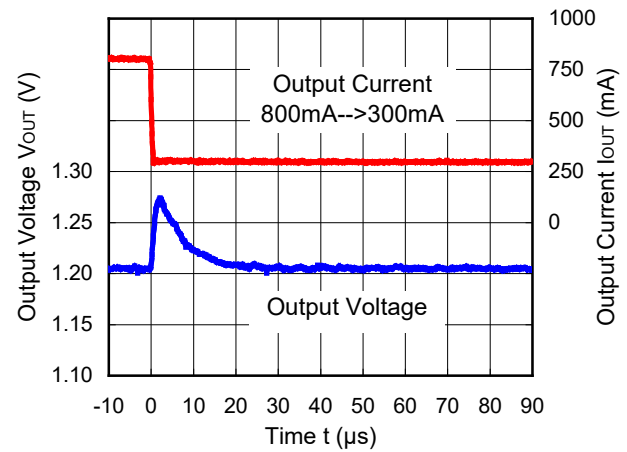
RP505K001C (V IN =3.6V, V OUT =1.2V)
