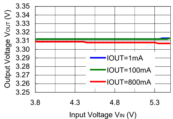
RP505K V_{OUT}=3.3V
