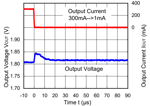
RP505K181A/B (V IN =3.6V) MODE="H" forced PWM
