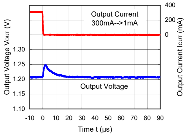
RP505K001C (V IN =3.6V, V OUT =1.2V) MODE="H" forced PWM
