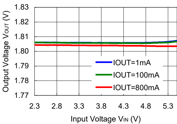
RP505K V_{OUT}=1.8V
