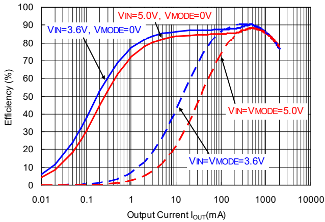
RP506Lxx1K/L/M V_{OUT} = 3.3\text{ V}
