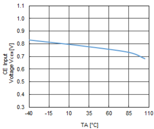
CE“H” Input Voltage ( V_{IN} = 5.5 V)
