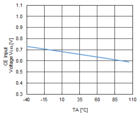
CE“L” Input Voltage ( V_{IN} = 2.5 V)
