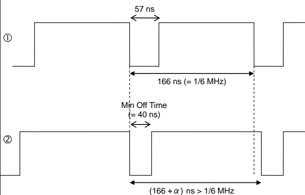
LX Waveform
