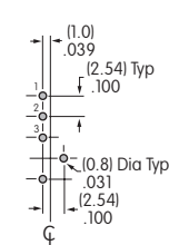
AB11 model does not have terminal 2. AB15AV-FA
