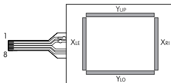
XLE, XRI: Top Electrode Terminal YUP, YLO: Bottom Electrode Terminal
