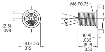
D4 6mm/.350" (8.9mm) Threaded with D Flat
