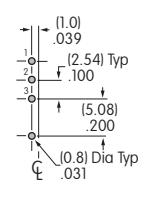
V1 Terminals
