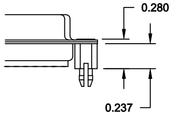
90X ..... 0.237" (BOARD SIDE) - CN10-237-093
