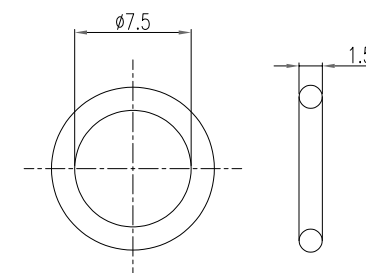
O-RING B
