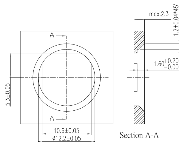
Panel Cut Out Recommendation
