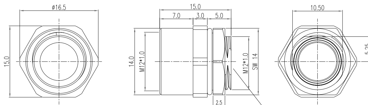
SHELL+O-RING A+NUT
