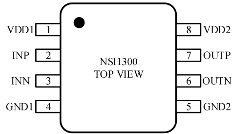
Figure 1.1 NSi1300 Package
