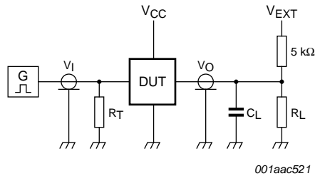
Test data is given in Table 10. Definitions for test circuit: RL = Load resistance. CL = Load capacitance including jig and probe capacitance. RT = Termination resistance should be equal to the output impedance Zo of the pulse generator. VEXT = External voltage for measuring switching times.
