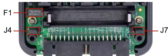
Figure 5. BATT-14AAAPACK Configurations
