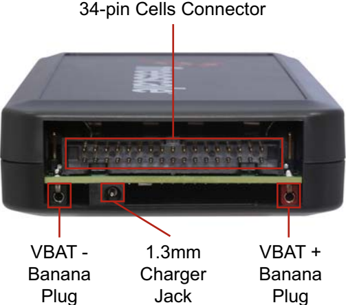
Figure 4. Side View
