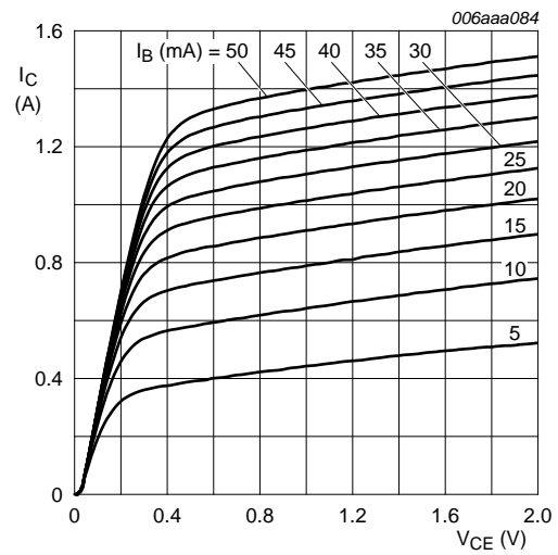
T_{amb} = 25^\circ\text{C}
