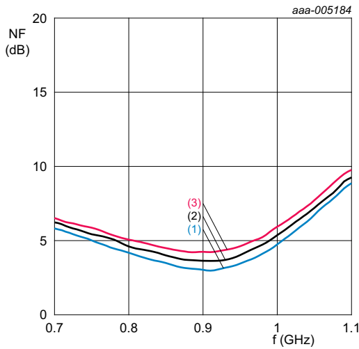
V_{SUP} = 3.6 V ; I_{CC(tot)} = 70 mA ; matched for ISM-915. (1) T_{amb} = -40 °C (2) T_{amb} = +25 °C (3) T_{amb} = +85 °C
