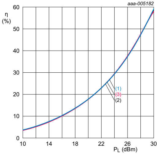
V_{SUP} = 3.6 V ; I_{CC(tot)} = 70 mA ; matched for ISM-915. (1) T_{amb} = -40 °C (2) T_{amb} = +25 °C (3) T_{amb} = +85 °C
