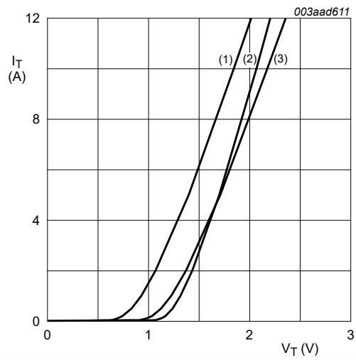
Fig. 10. On-state current as a function of on-state voltage V_o = 1.27\text{ V}; R_s = 0.091\ \Omega
