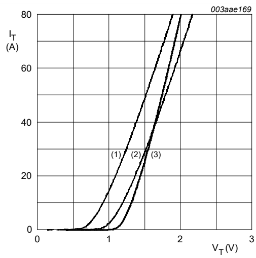
V_o = 1.073 \text{ V}; R_s = 0.015 \Omega (1) T_j = 125^\circ\text{C} ; typical values (2) T_j = 125^\circ\text{C} ; maximum values (3) T_j = 25^\circ\text{C} ; maximum values Fig. 10. On-state current as a function of on-state voltage
