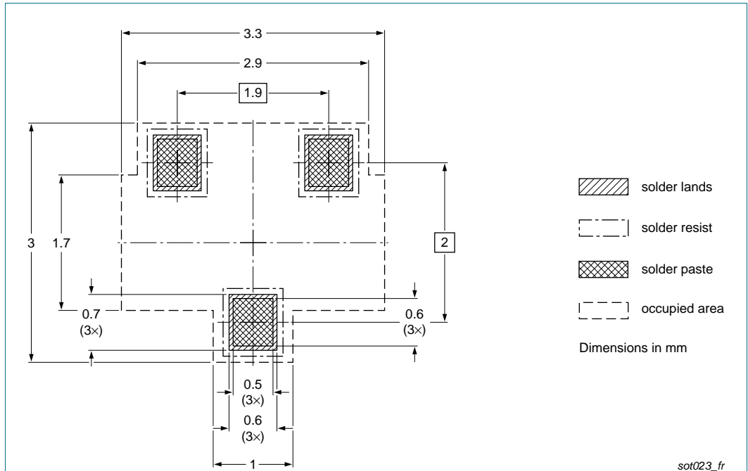
Fig 9. Reflow soldering footprint SOT23 (TO-236AB)
