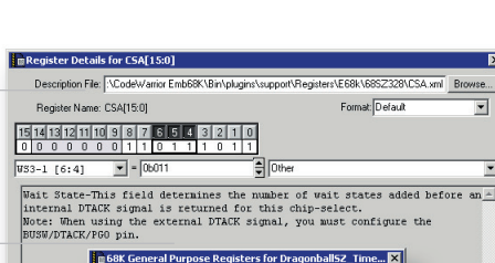
General Purpose Registers
