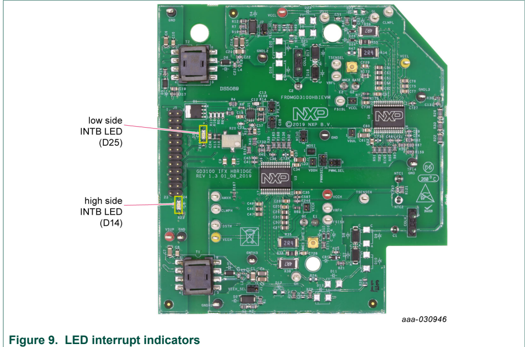
Figure 9. LED interrupt indicators
