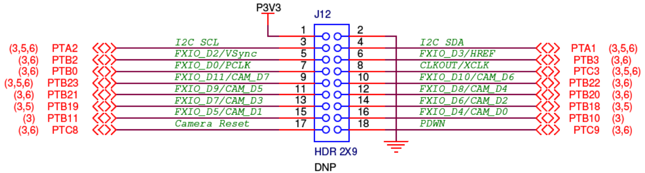
Figure 12. FlexIO/camera header
