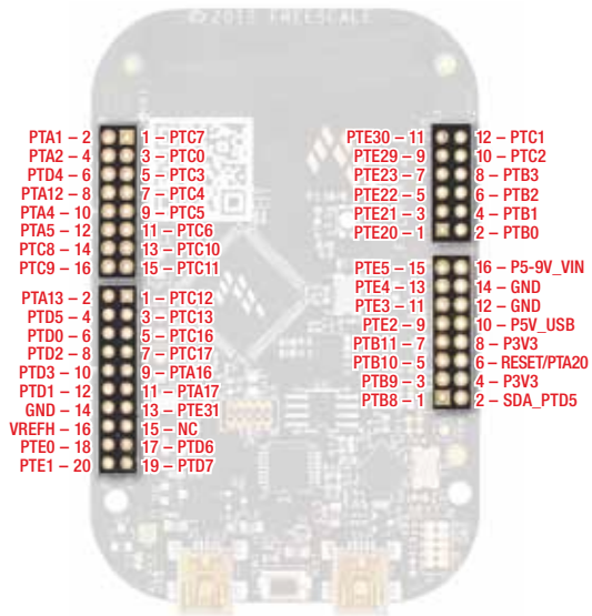
Figure 2: FRDM-KL25Z Pin-Out
