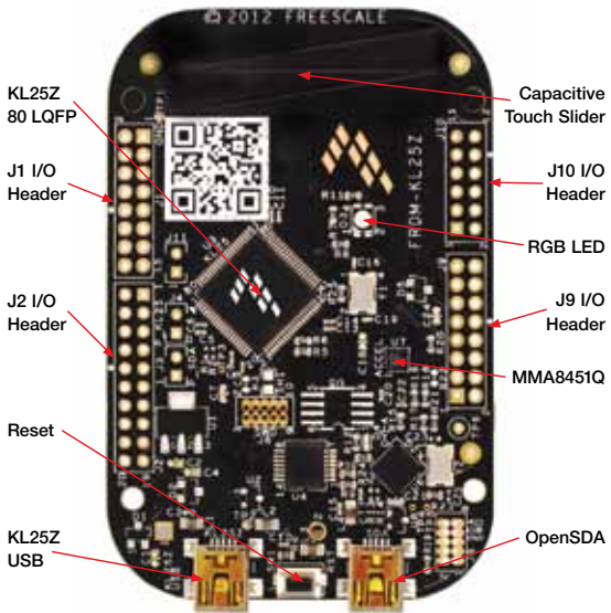
Figure 1: FRDM-KL25Z Callouts
