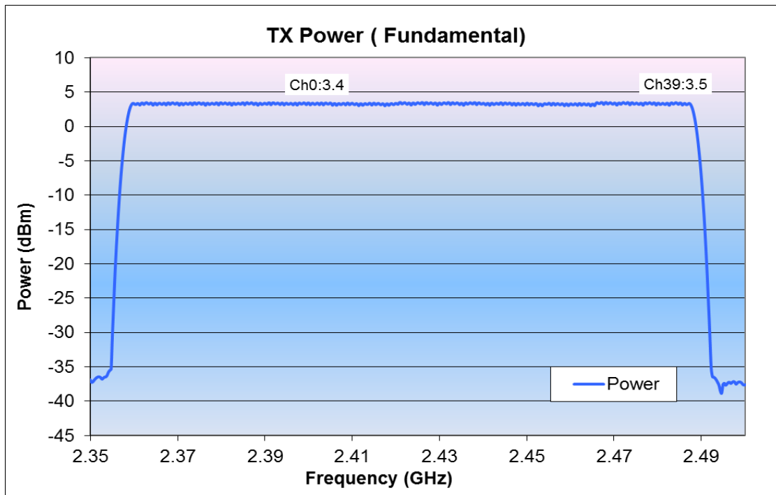
Figure 7. TX power
