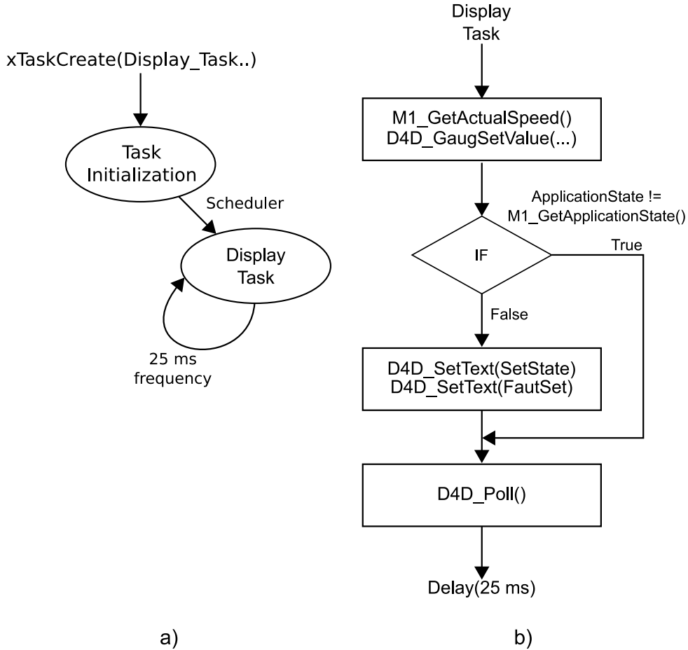
Figure 16. Display_Task flowchart
