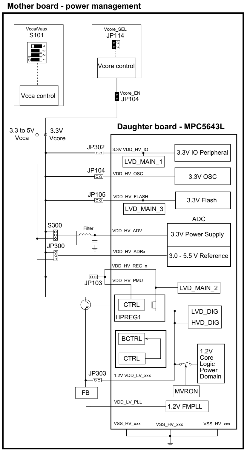
Figure 11. MPC5643L Power Supply Scheme
