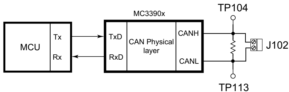
Figure 9. CAN Interface
