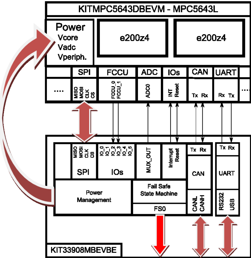
Figure 2. Interfacing with the KIT33908MBEVBE
