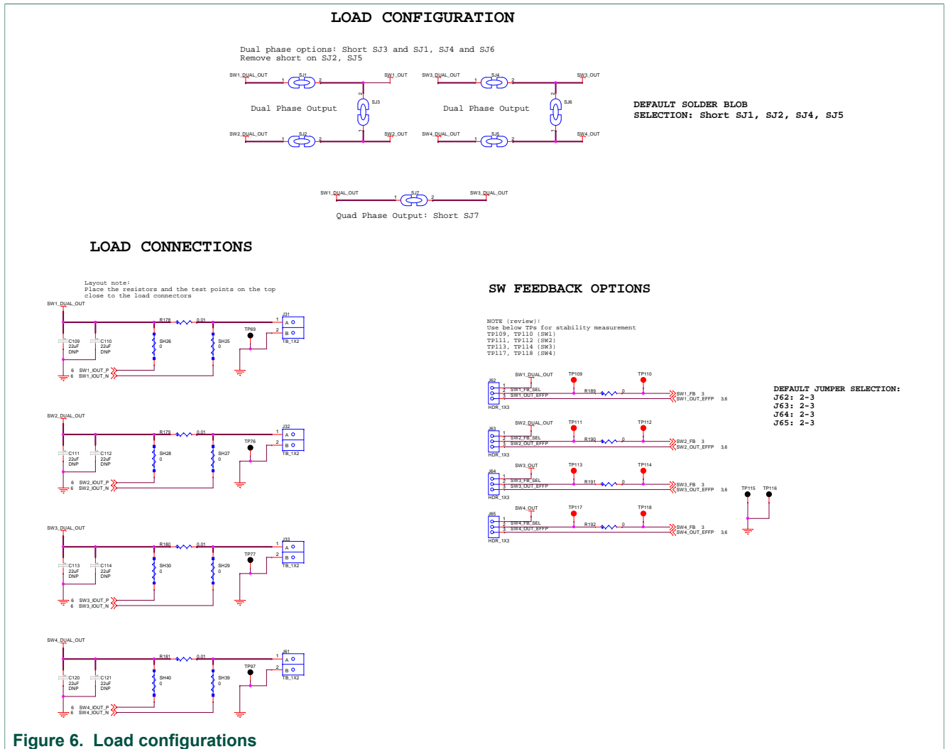
Figure 6. Load configurations
