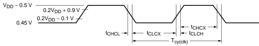
Fig 7. External clock timing
