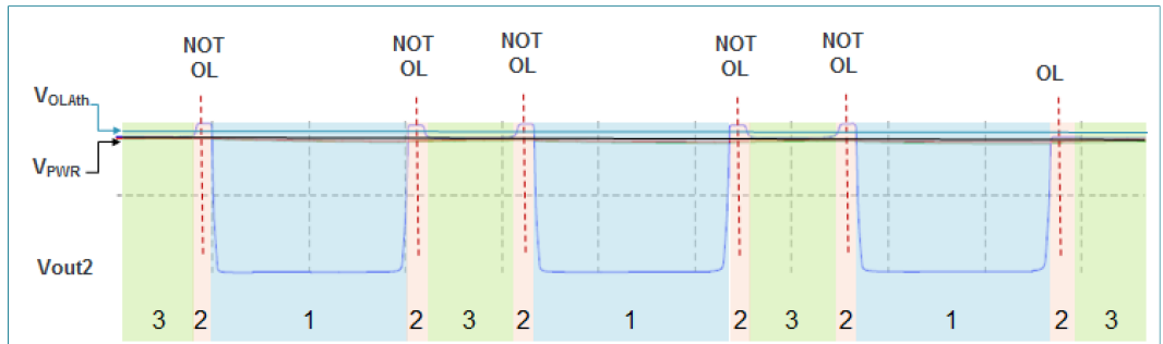
Figure 16. Open load circuit operation
