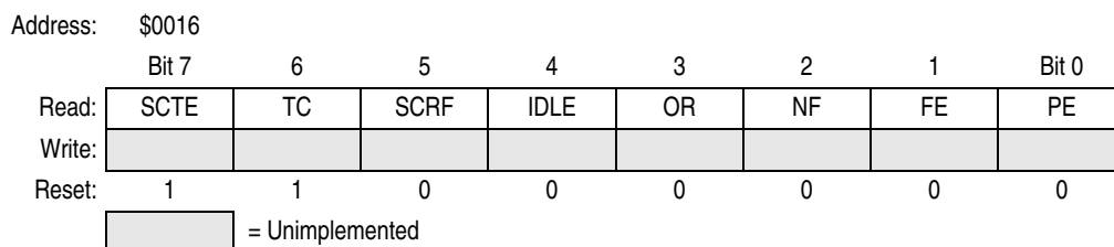
Figure 15-13. ESCI Status Register 1 (SCS1)
