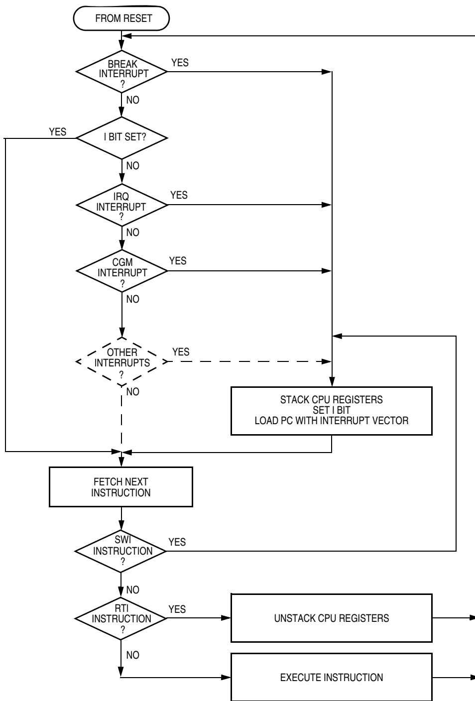
Figure 14-5. Interrupt Processing
