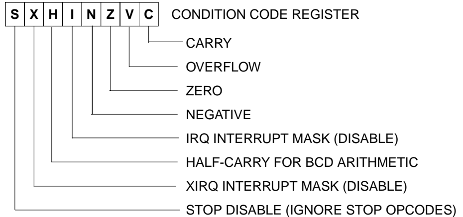
Figure 1 Programming Model
